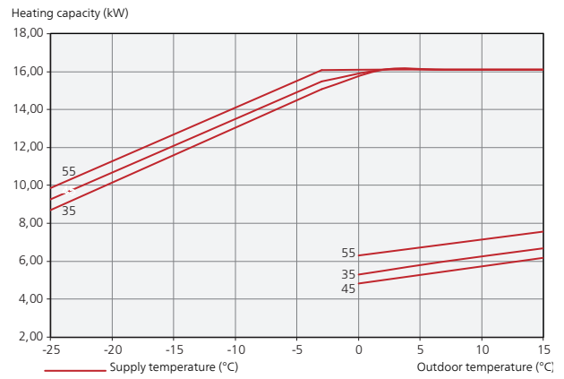
JÄSPI Inverter Nordic-20 max and min heating capacity
