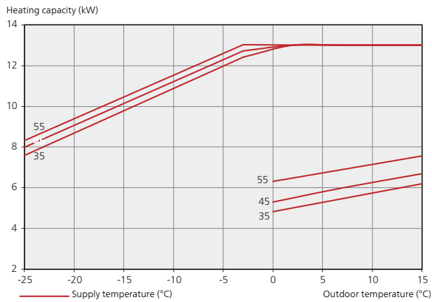
JÄSPI Inverter Nordic-16 max and min heating capacity
